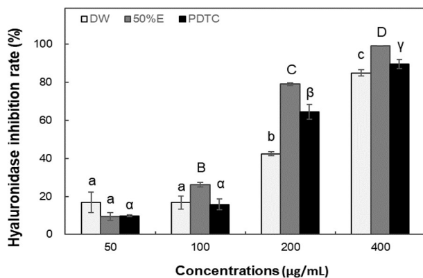
Fig. 6. Hyaluronidase inhibition activity of Aeonium sedifolium . Values are presented as mean \pm standard deviation (n=6). Means with the letters (a-d) above the bars are significantly different at p < 0.05 , as determined by Duncan's multiple range test.
