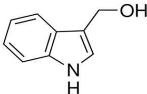
Fig. 1. Chemical structure of indole-3-carbinol.
