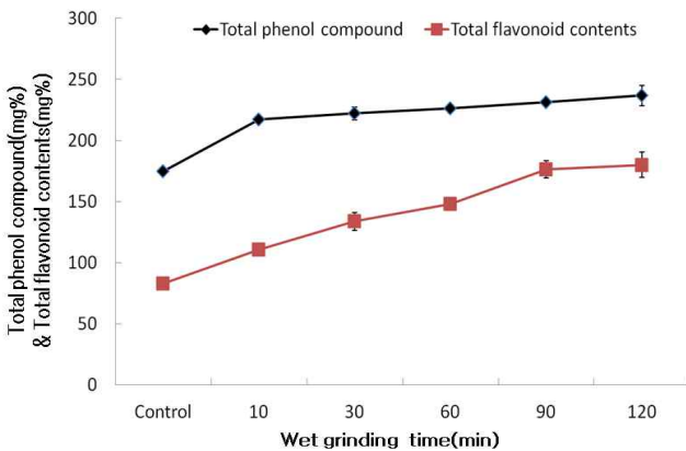
Fig. 1. Total phenol compound and total flavonoid contents of whole buckwheat powder by wet grinding time.
