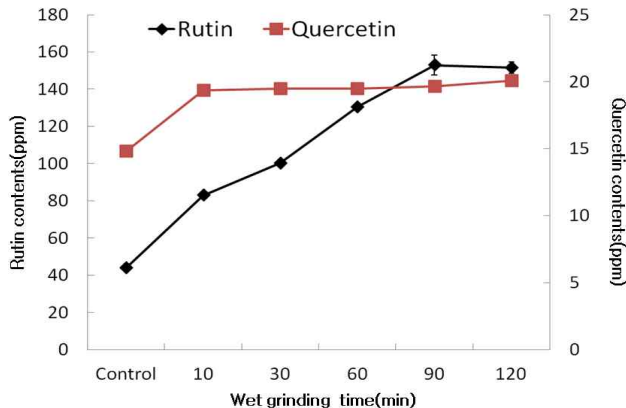
Fig. 2. Rutin and quercetin contents of whole buckwheat powder by wet grinding time.
