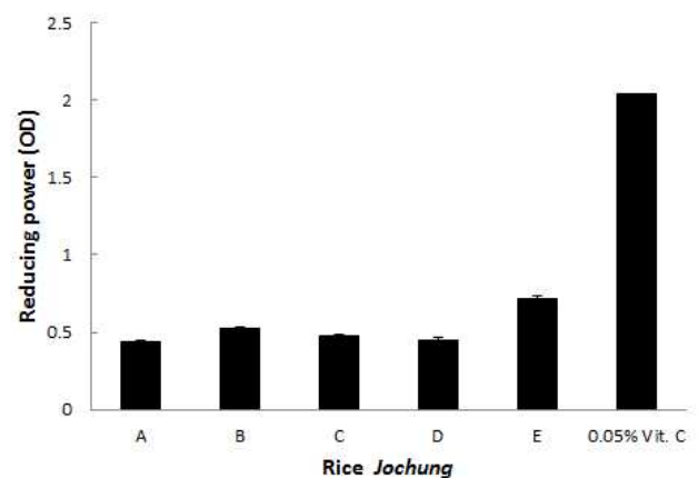
Fig. 2. Reducing power of various rice Jochung products.
