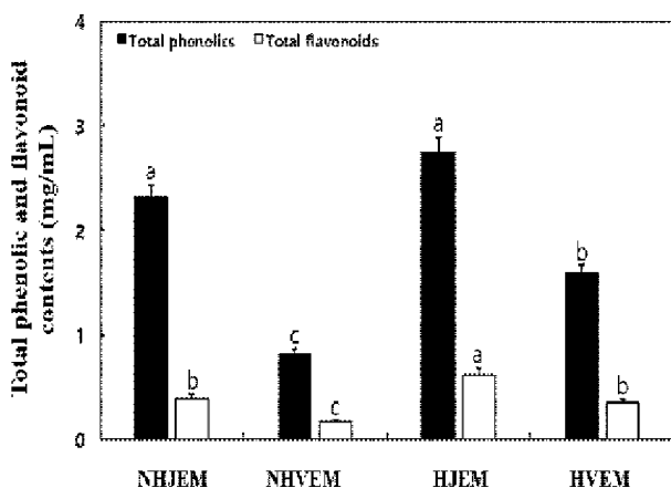
Fig. 2. Comparison of the total phenolic and flavonoid contents of the juices and vinegars from Elaeagnus multiflora fruit.
